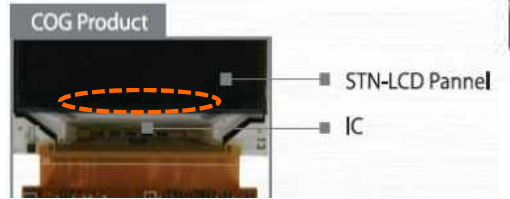
COG bonding [IC / LCD]
