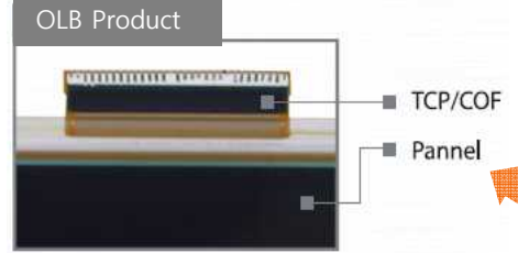
TAB bonding_Input [TCP / LCD]
